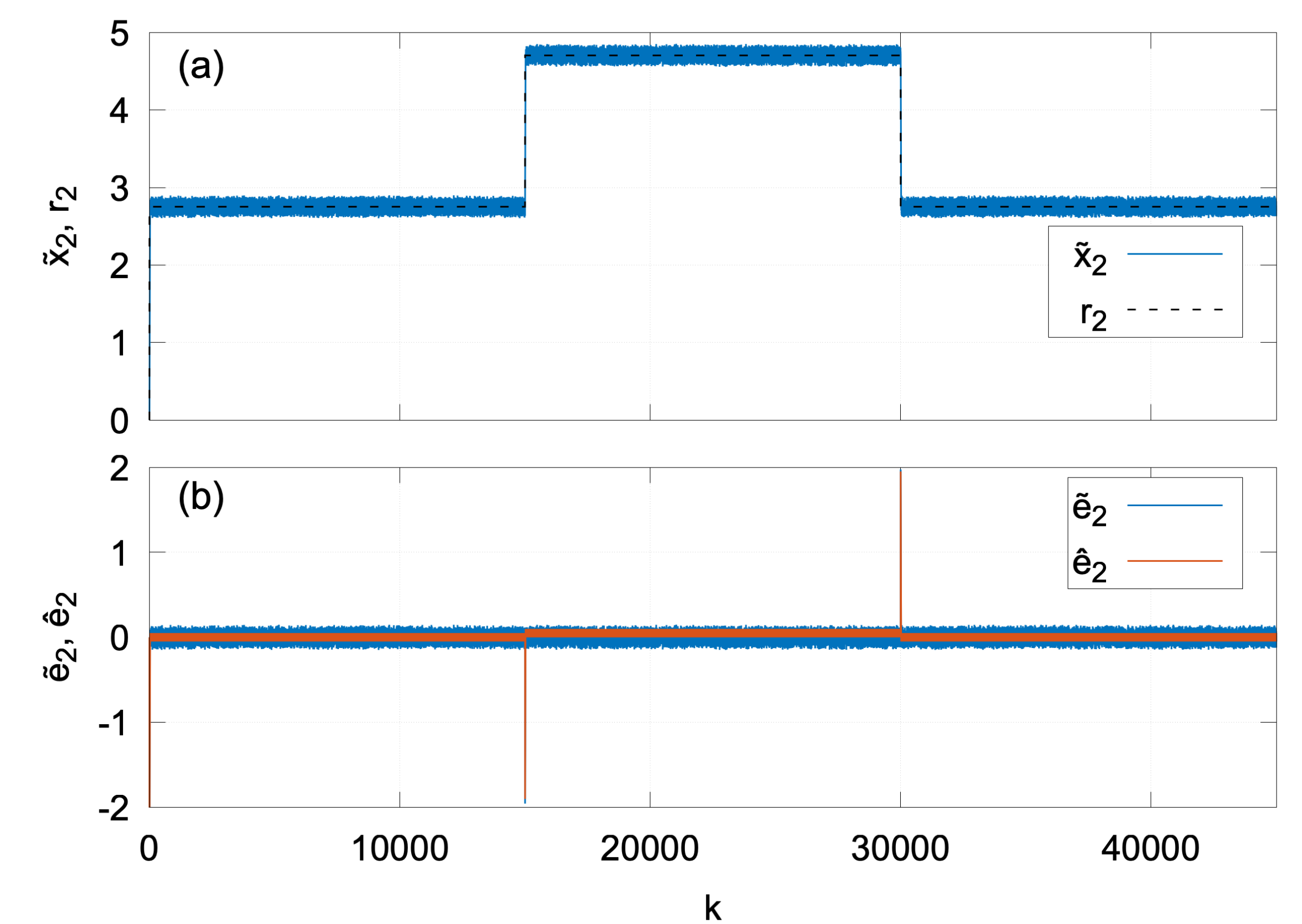
Fig. 2. CSTR closed-loop response under additive stochastic attack, with the tilde marking perturbed quantities and the hat marking defended quantities: (a) perturbed state \tilde{x}_2 against reference r_2 ; (b) perturbed tracking error \tilde{e}_2 and defended tracking error \hat{e}_2 over n = 45,000 iterations.
