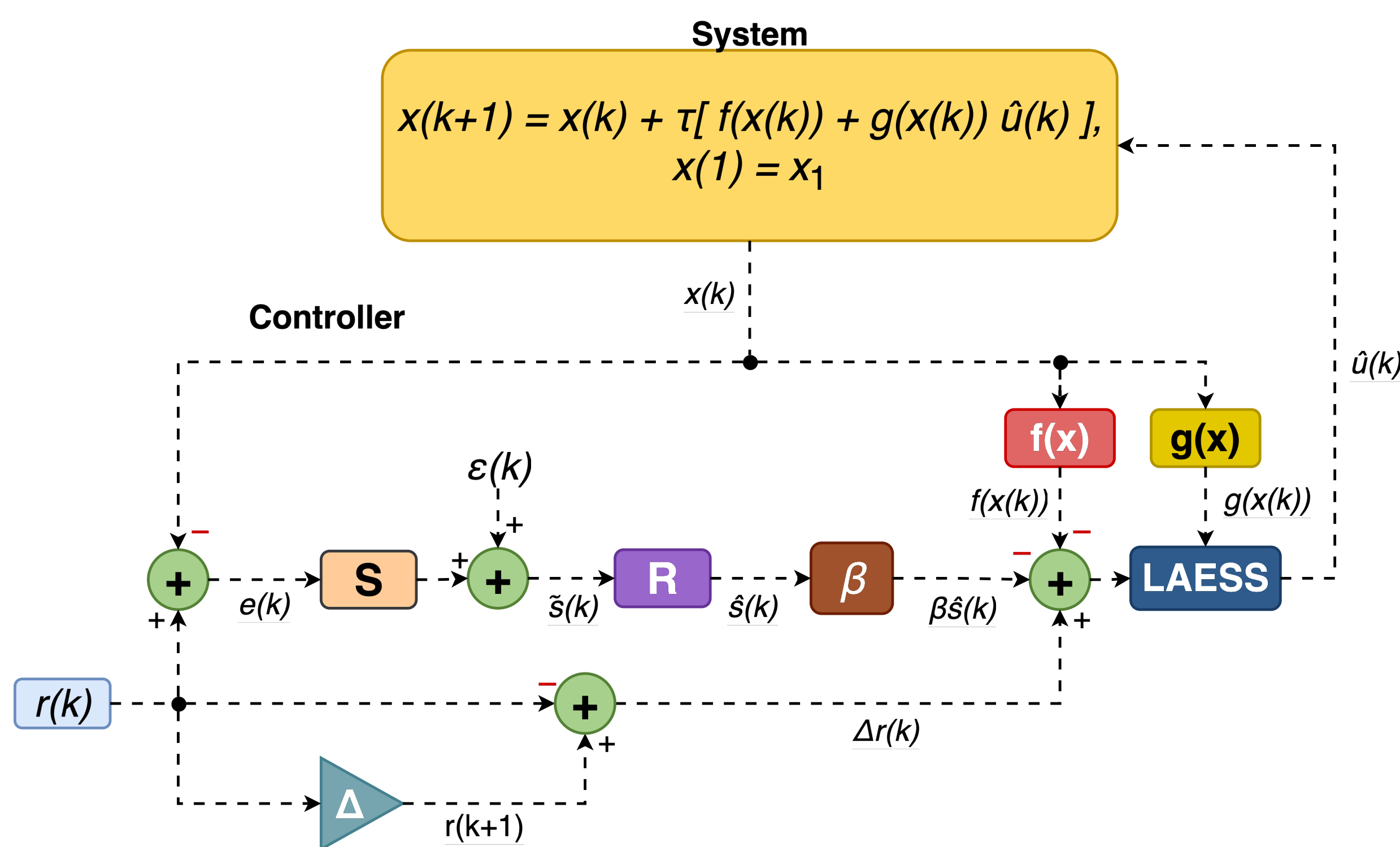
Fig. 1. Functional block diagram of the defended closed-loop system. The block S computes \operatorname{sgn}(e(k)) , \epsilon(k) is the zero-mean Gaussian disturbance, R is nearest-integer rounding, \Delta forms r(k+1) - r(k) , and LAESS applies the control law using f , g , and \beta .
